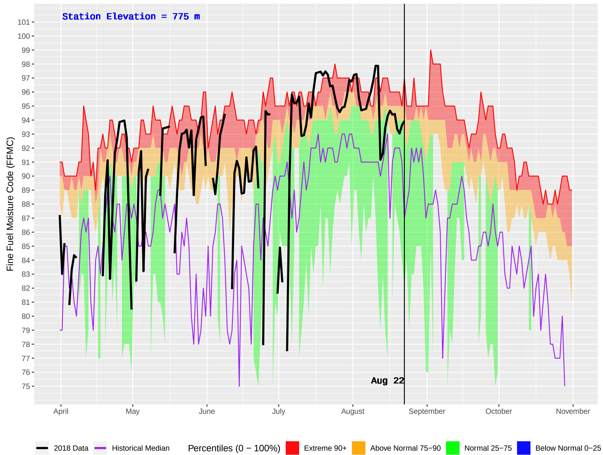
ELKO (412) : Historical (1970–2016) and Current (2018) Daily Fine Fuel Moisture Code (FFMC)
