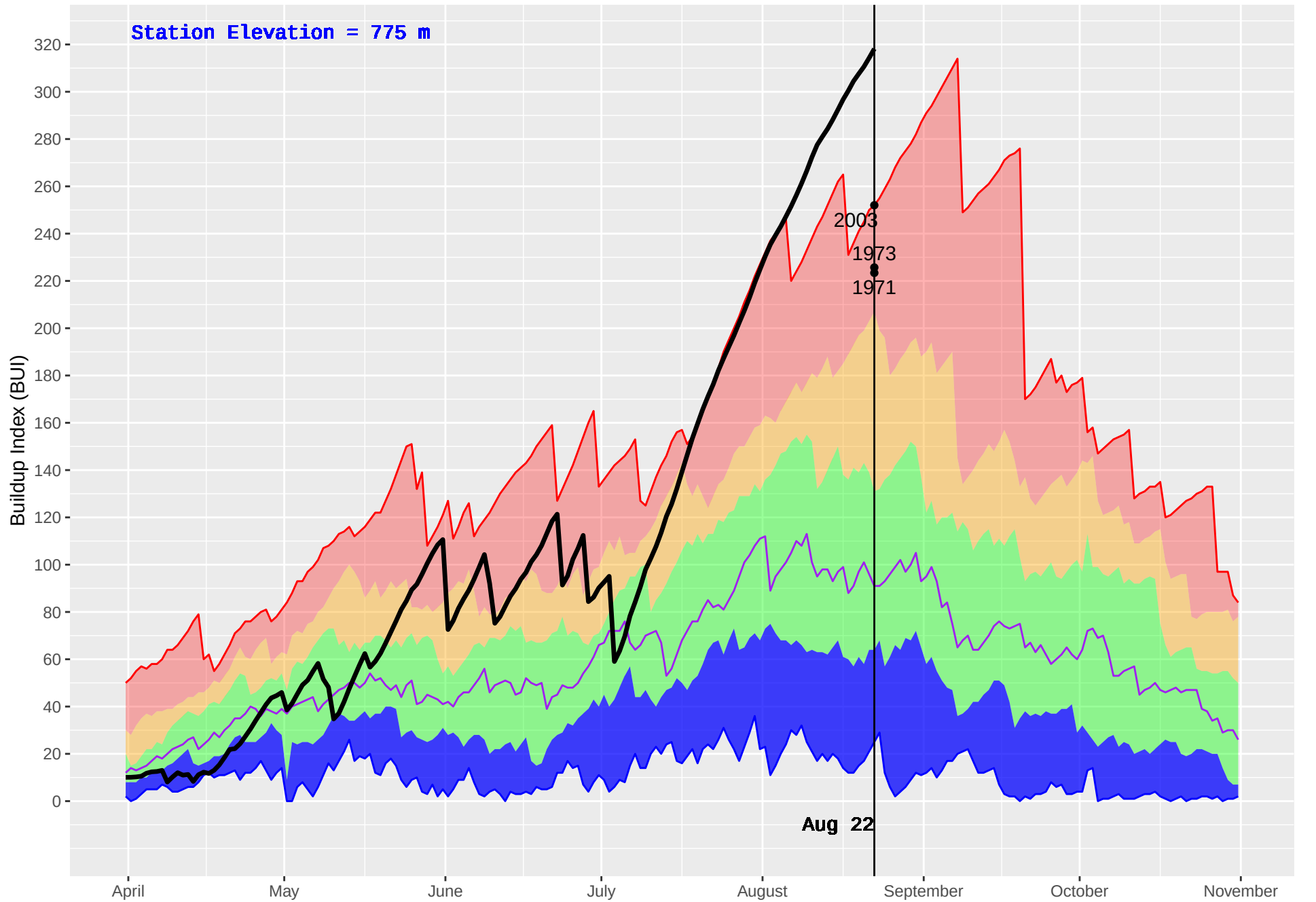
ELKO (412) : Historical (1970–2016) and Current (2018) Daily Buildup Index (BUI)
